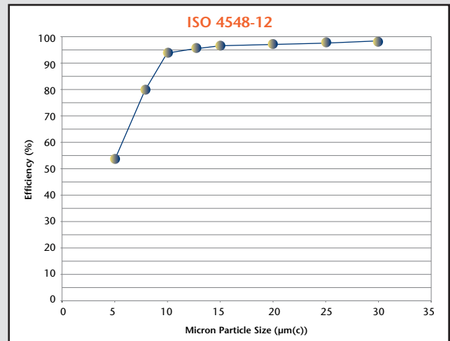
Particle Removal Efficiency vs. Particle Size Test after Test after Test...
