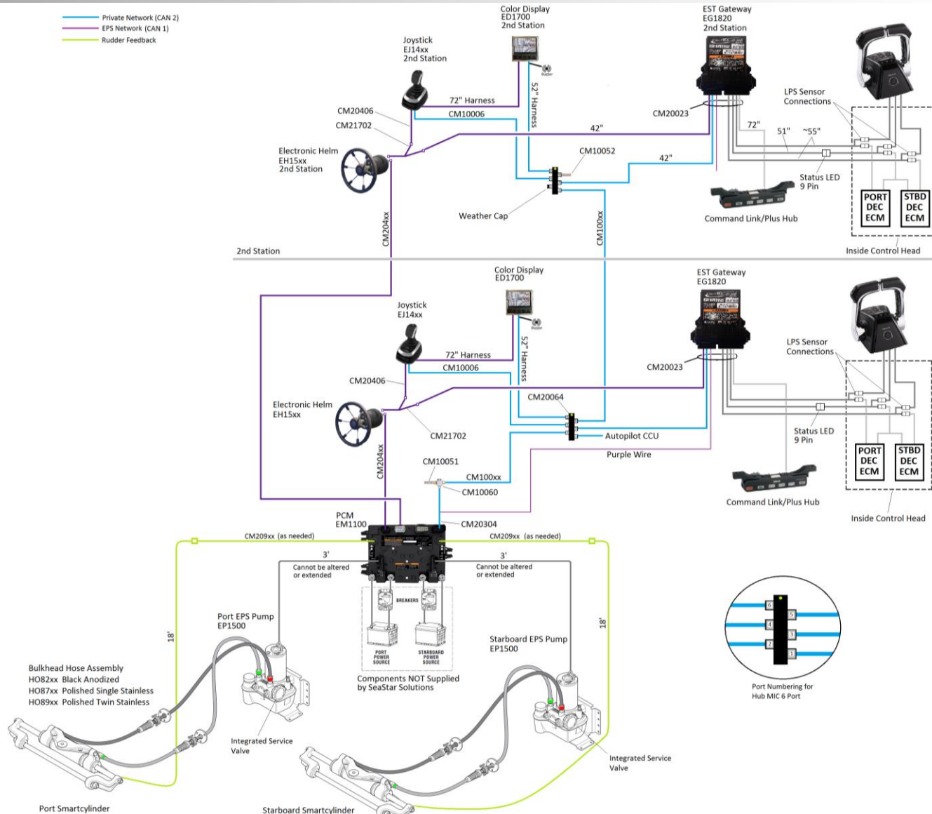
Optimus 360 - Yamaha DEC - Dual Station, Twin Engine
