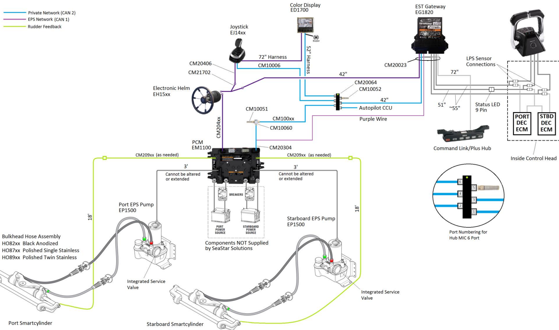
Optimus 360 - Yamaha DEC - Single Station, Twin Engine
