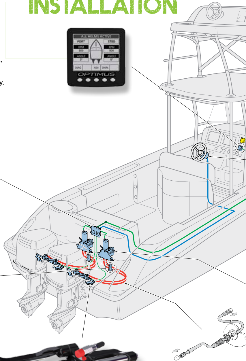
Hydraulic Lines
