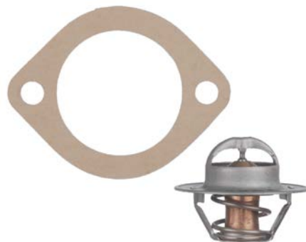
23-3661 THERMOSTAT KIT Temperature Rating: 140° Replaces: Westerbeke 35736 & 40434 Fits: 20.0 BEG(60Hz)/16.0 BEG(50Hz), 25.0 BEG(60Hz)/20.0 BEG(50Hz)
