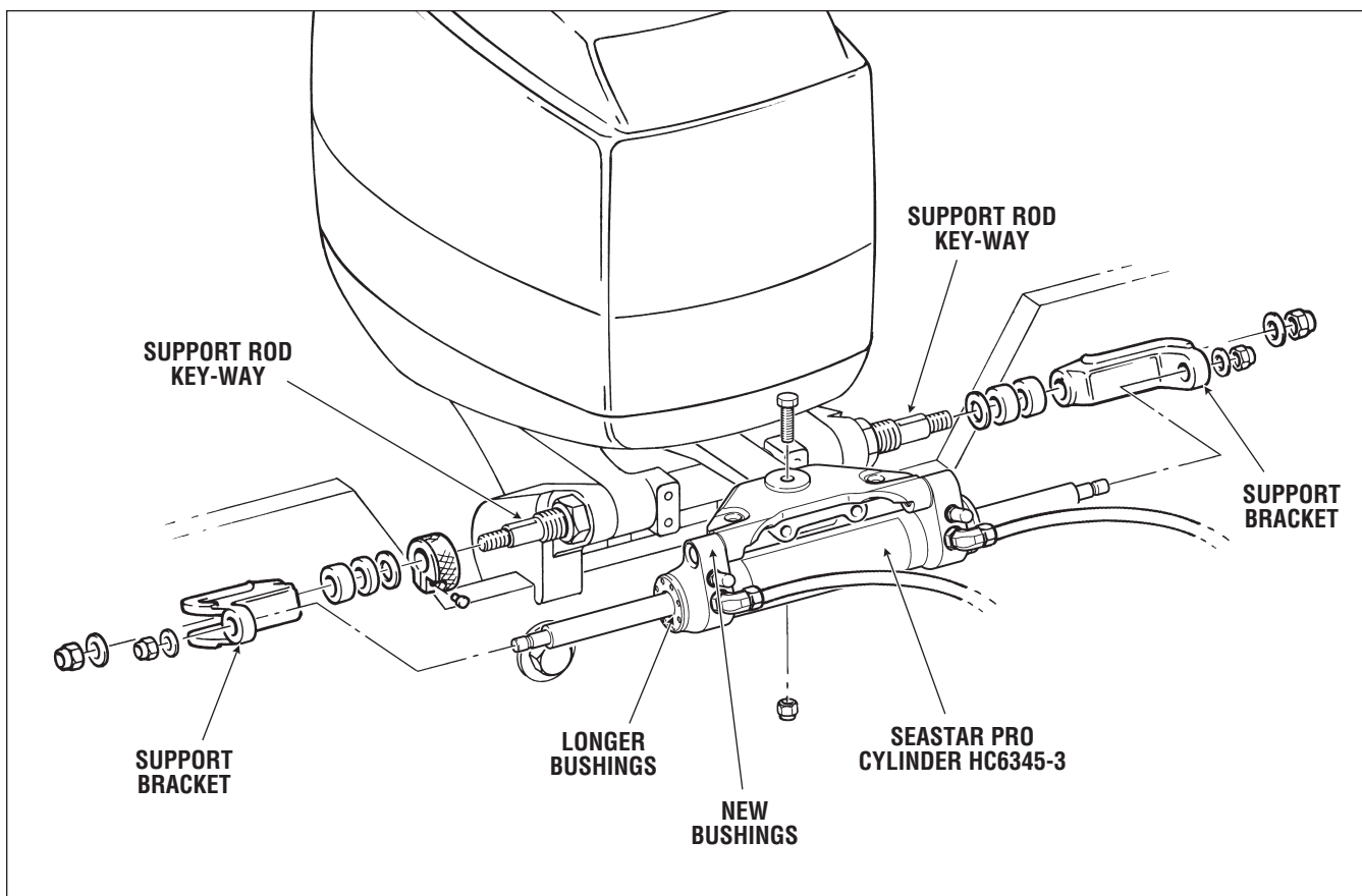
Cylinder Part# HC6345-3 shown.
