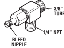
HF5532 Connector Fitting
