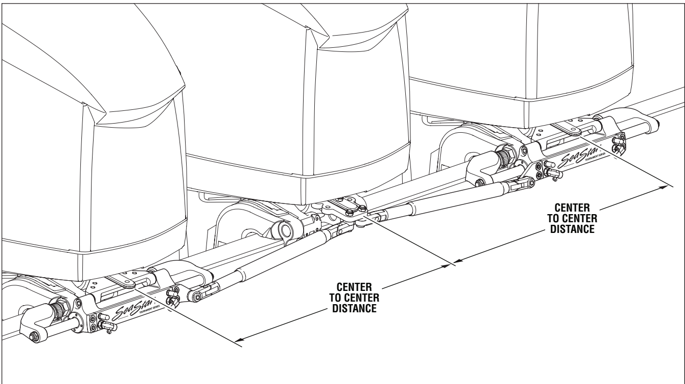
Triple Engine – Dual Cylinder Configuration.
