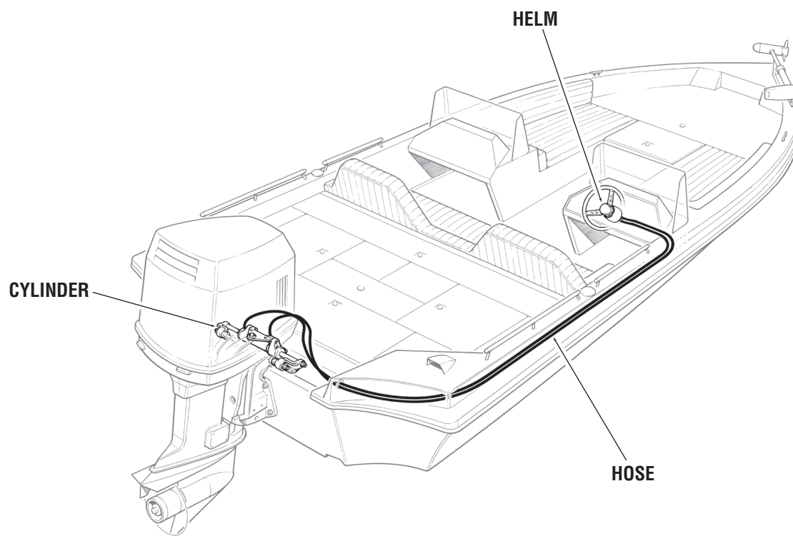
Typical SeaStar Installation.
